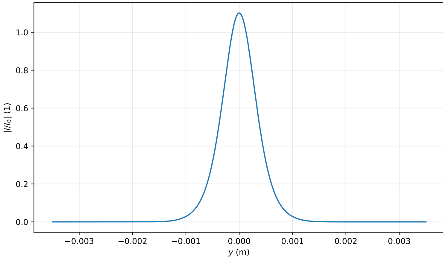
Intensity profile I(x=0, y, z=1.274)/I_0 , P_{in}=0.6P_{cr} , artificial time
